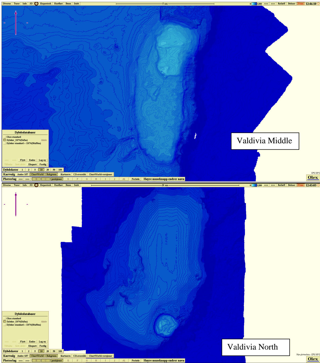
Figure 37. Bathymetry of the four subareas indicated in Figure KK1.
