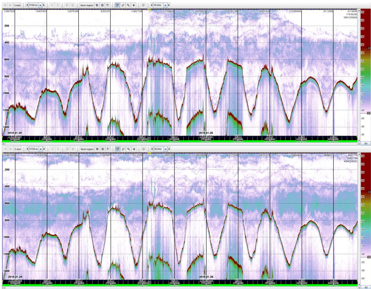
Figure 25. Echograms from acoustic survey of the Wüst Location 2. The map shows the track of the vessel during multiple crossings of the seamount during a 24 hour period. Echograms show results from 18 Khz (top) and 38 Khz (bottom) transducers.
