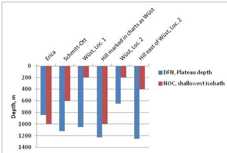
Figure 5. Comparison for a range of SE Atlantic seamounts between expected summit depths based on published bathymetries (mainly GEBCO data) (red bars) and measured summit plateau depths observed by Dr Fridtjof Nansen 2015 (blue bars).
