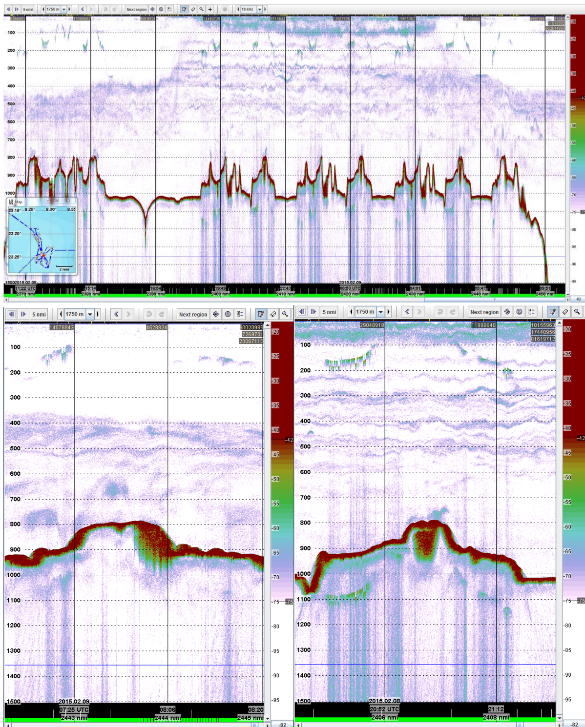
Figure 58. Echograms from the summit of Ewing seamount (EK60, 18 KHz). Composite from repeat crossings (“butterfly-survey”, upper graph), and details from day (lower left) and night (lower right) crossing.
