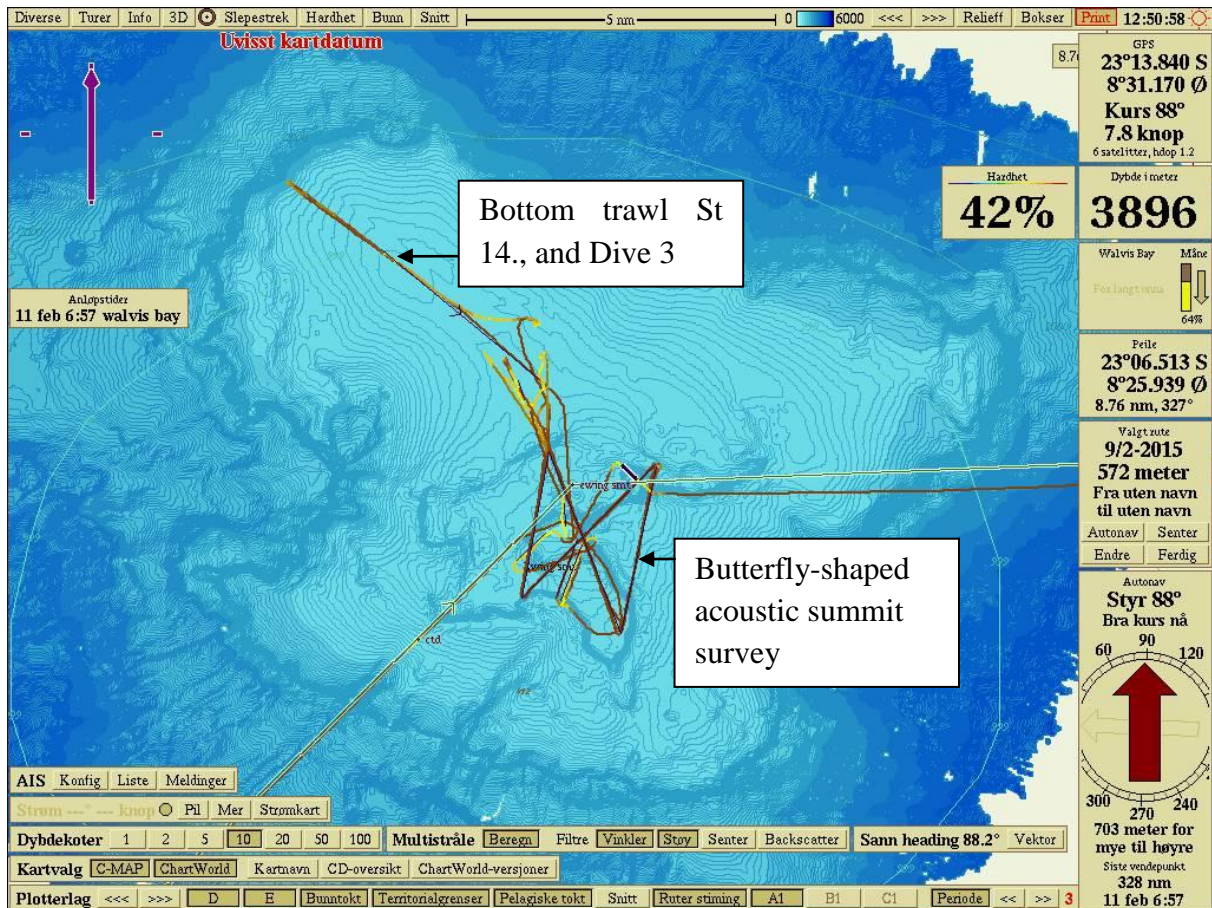
Figure 57. Vessel track on the Ewing Seamount, illustrating dive and trawl tow on the deep northwestern plateau, and the acoustic survey on the shallow summit.
