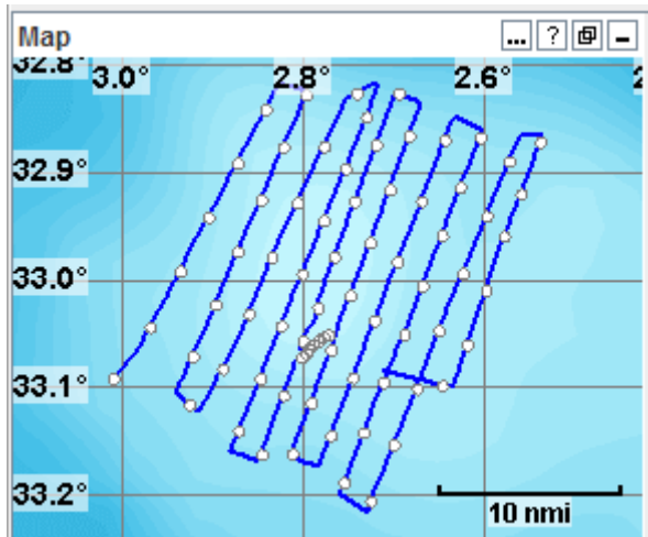
Figure 25. Echograms from acoustic survey of the Wüst Location 2. The map shows the track of the vessel during multiple crossings of the seamount during a 24 hour period. Echograms show results from 18 Khz (top) and 38 Khz (bottom) transducers.
