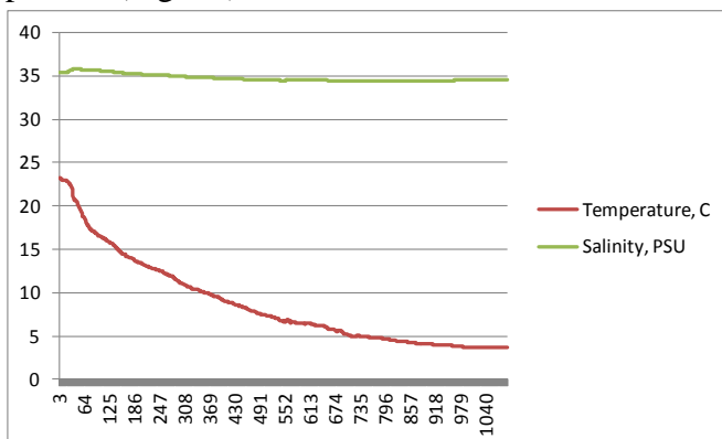
Figure 54. Depth profiles of temperature and salinity at Ewing Seamount, 23° 16.50 S, 008° 13.97 E on 8 February 2015
