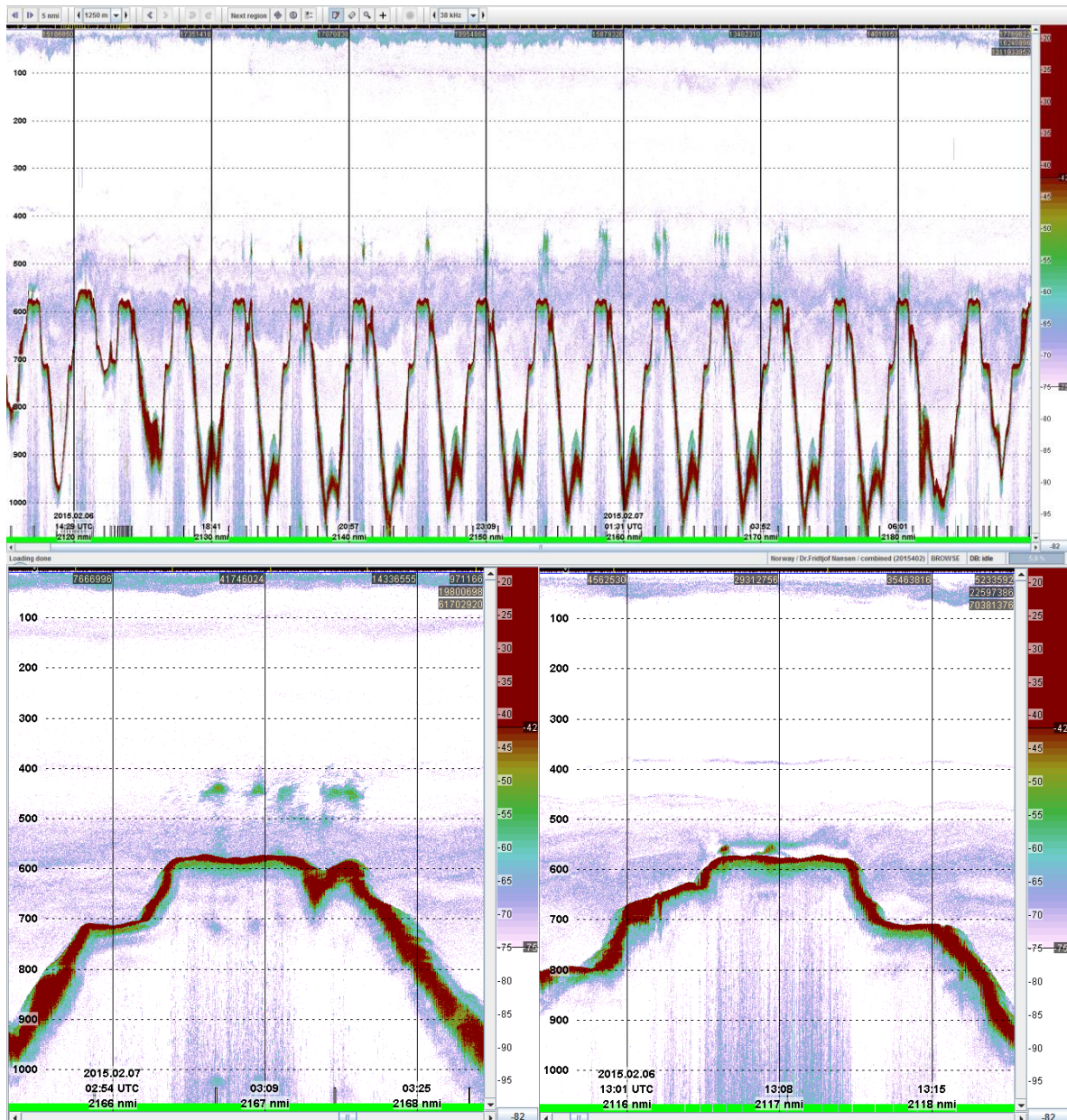
Figure 52. Echograms from 18-hour repeat study of an aggregation of fish above the Valdivia North seamount summit (EK60, 38KHz). Upper figure: full time-series starting at 13:00 UTC (15:00 local time) on 6 February and ending at approx. 07:00 UTC on the next day; Lower left: detailed echogram from nighttime (02-03UTC), Lower right: same from daytime (13:00 UTC).
