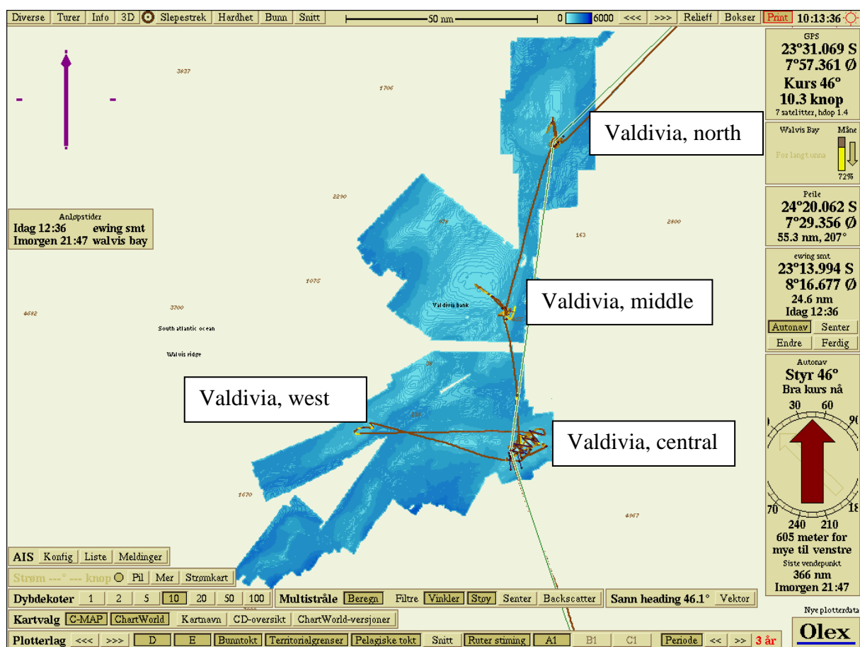
Figure 36. Valdivia Bank and surrounding seamounts on the Walvis Bay. The Dr Fridtjof Nansen visited the four subareas as indicated. Detailed bathymetries of each subarea are provided in Figure 37. Blue area with isobaths has been mapped by multibeam echosounders (see text). Red lines are tracks of the RV DFN.
